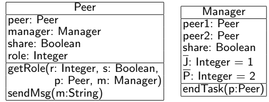
Fig. 1 Example: UML Class Diagram
