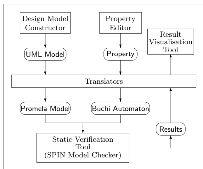
Fig. 3 UML Static Verification Framework
